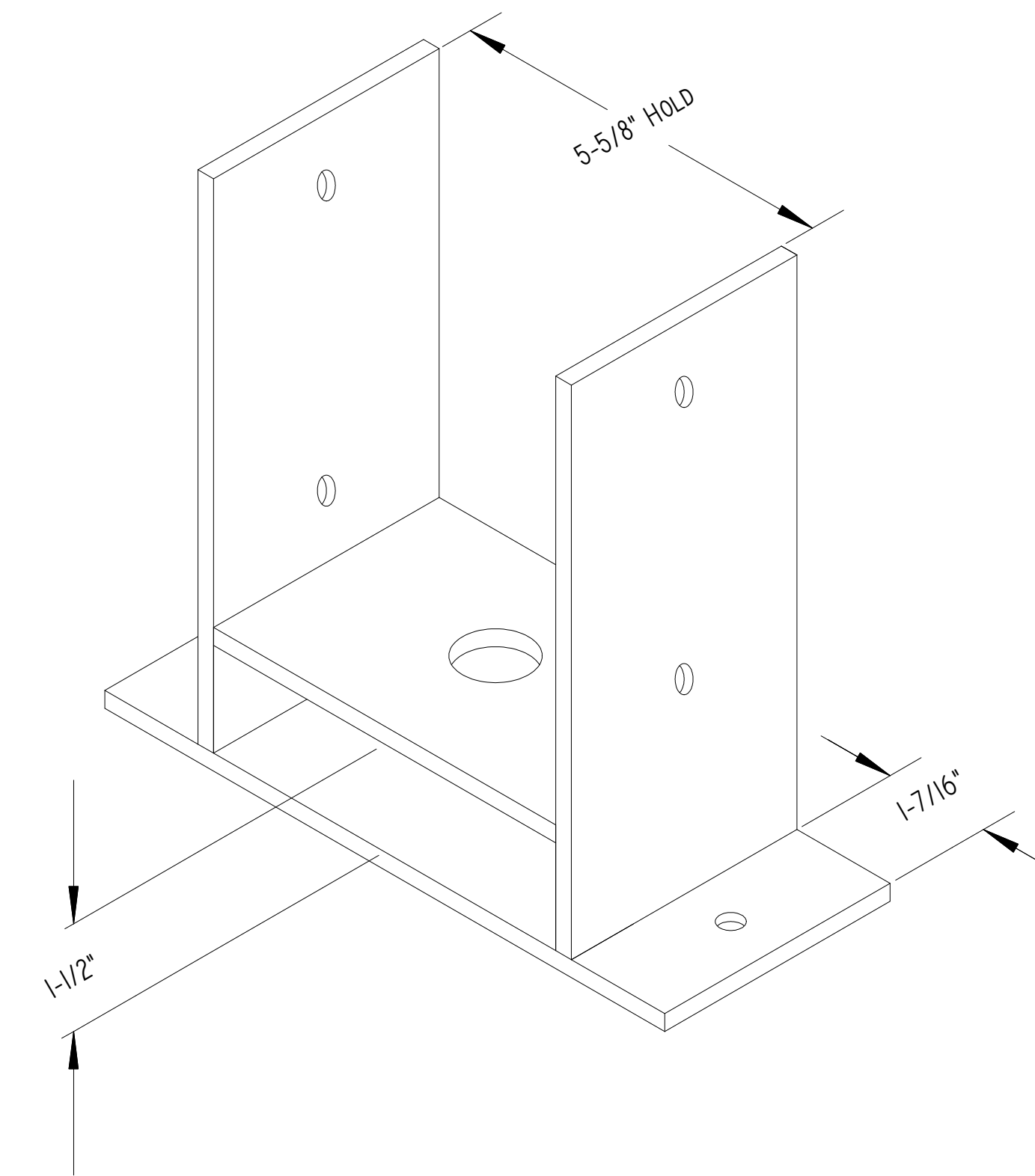
WELDMNT ASSY. CONTINUOUS WELD E7018
